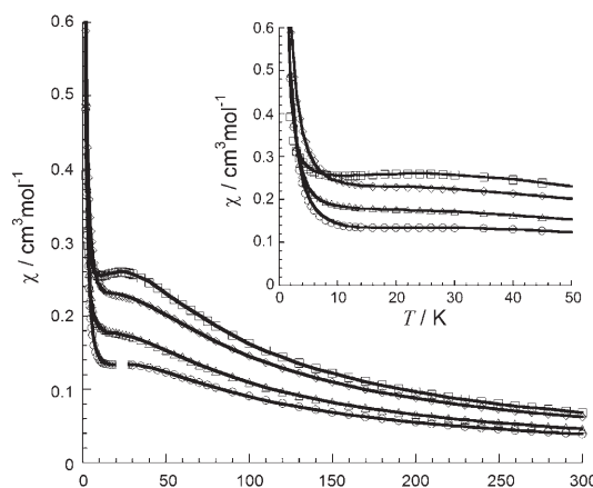
Figure 5. Variable-temperature behavior of \chi_{\text{m}} for 2 ( \square ), 3 ( \diamond ), 4 ( \circ ), and 5 ( \triangle ). All compounds were measured in a 0.1-T field. Solid lines: fit of data using set A parameters from Table 1. The inset shows an expansion of the curves for the low-temperature region.
